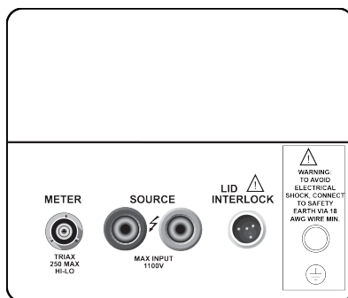
Figure 3: Side view - connectors
