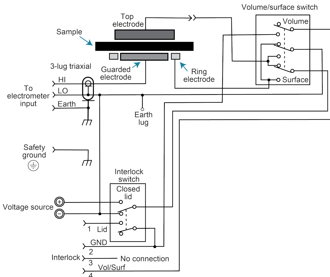
Figure 4: 8009 schematic diagram
