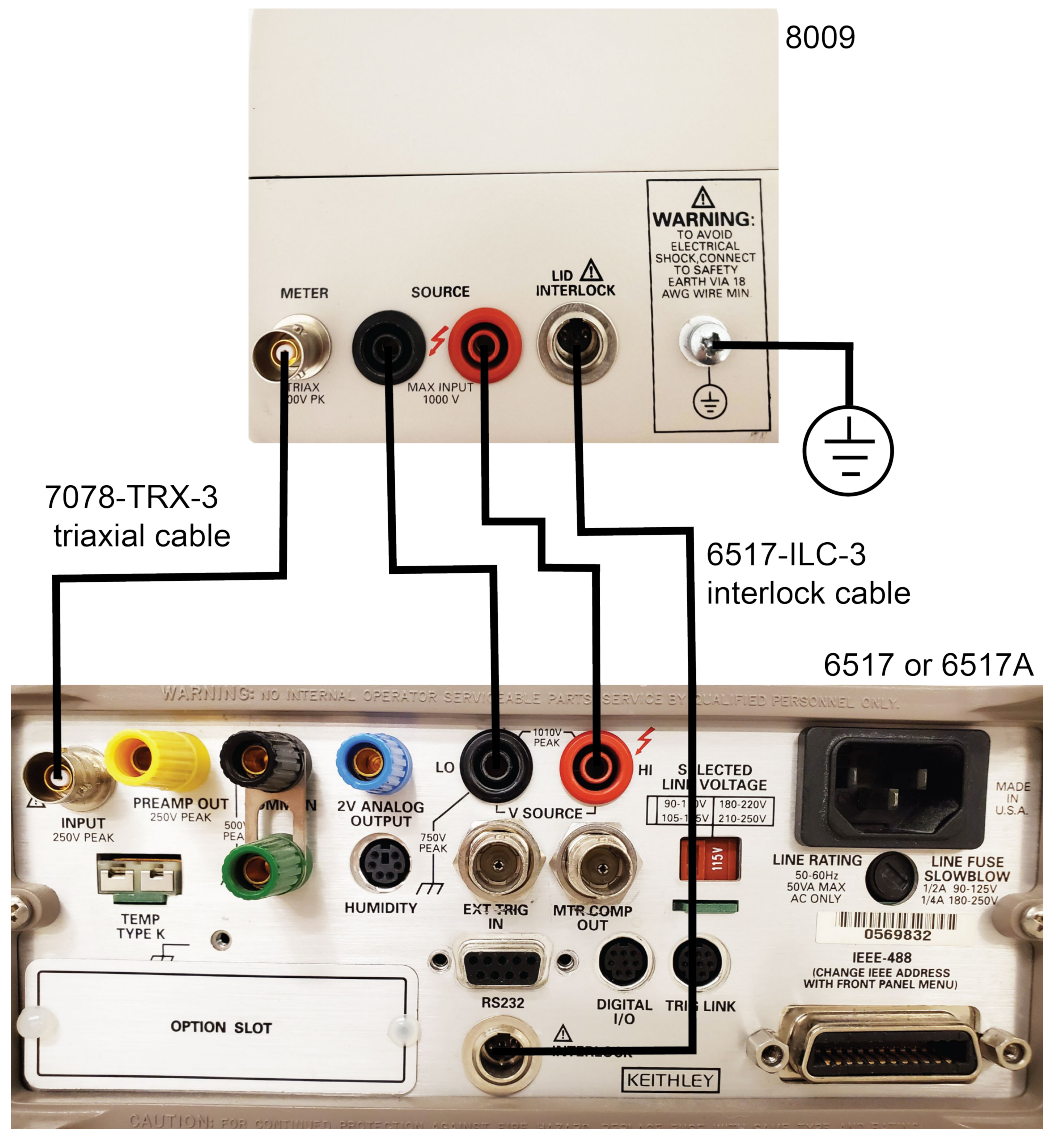
Figure 5: Connecting a 6517 to the 8009
