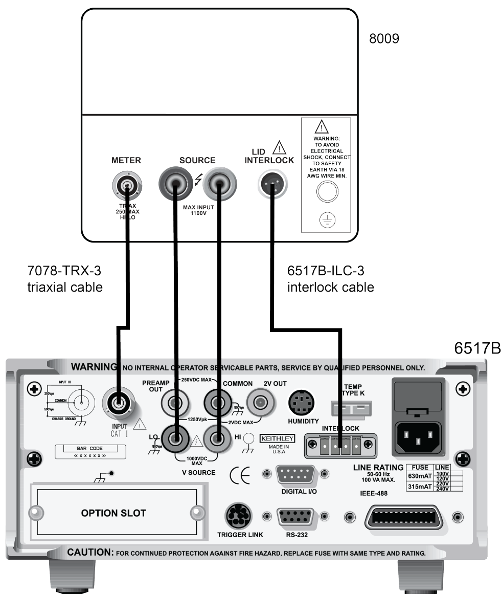
Figure 6: Connecting a 6517B to the 8009
