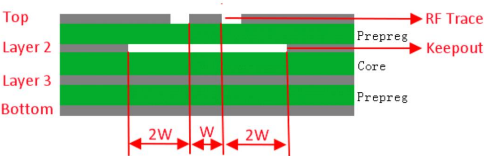
Figure 4: Schematic diagram of the four-layer board LAYOUT (the reference ground is the third layer)
