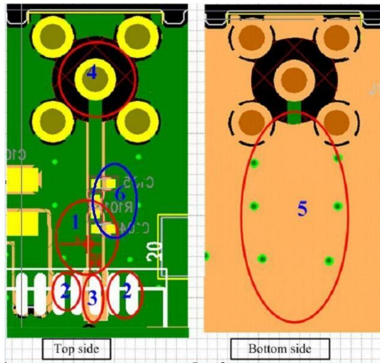
Figure 6: PCB LAYOUT
