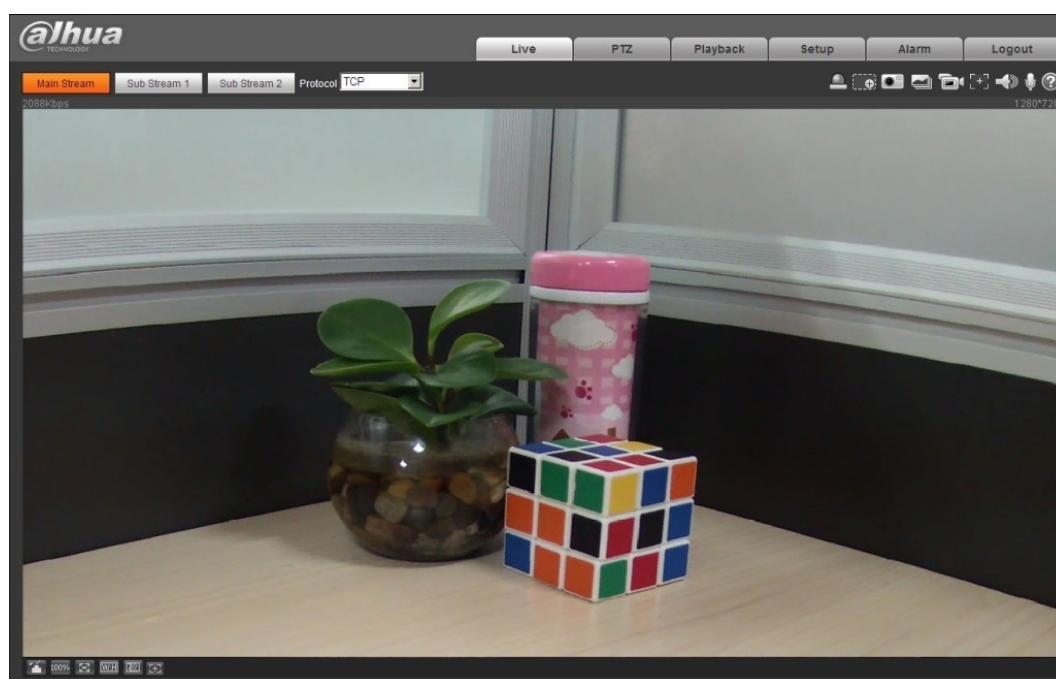
Figure 2-4 Main interface
