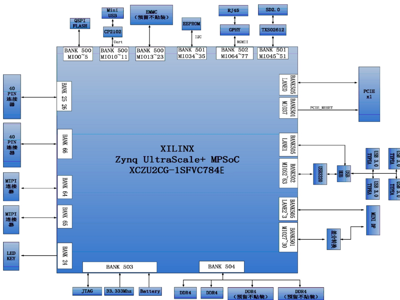
Figure 1-1: Board Schematic
