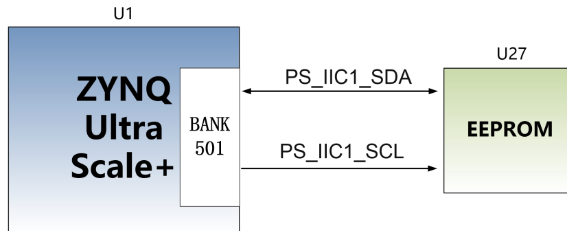
Figure 6-1: EEPROM Schematic
