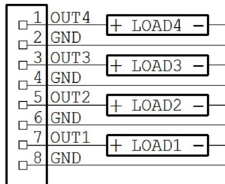
0-10V OUTPUTS CONFIGURATION. MAX LOAD = 10mA
