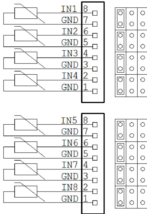
TEMPERATURE MEASUREMENT CONFIGURATION WITH 10K THERMISTORS
