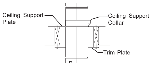
FIG. 3 CEILING SUPPORT
