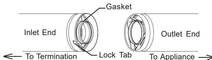
FIG. 2 JOINT CONNECTION
