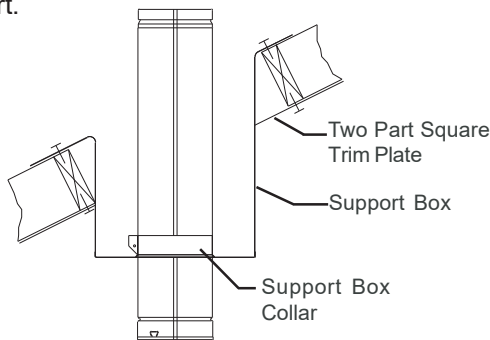
FIG. 4 SUPPORT BOX
