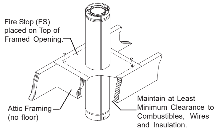
FIG. 6 FIRESTOP SPACER
