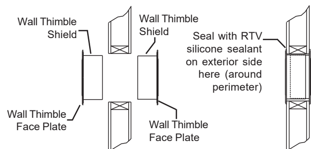
FIG. 9 WALL THIMBLE
