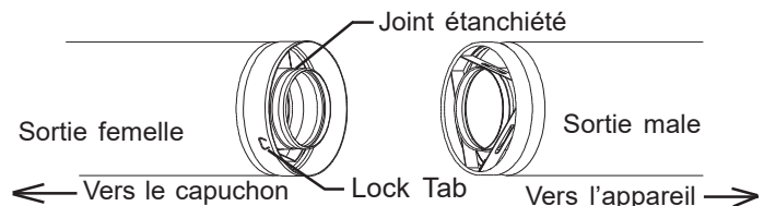
Schéma 2 - Raccordement de joint
