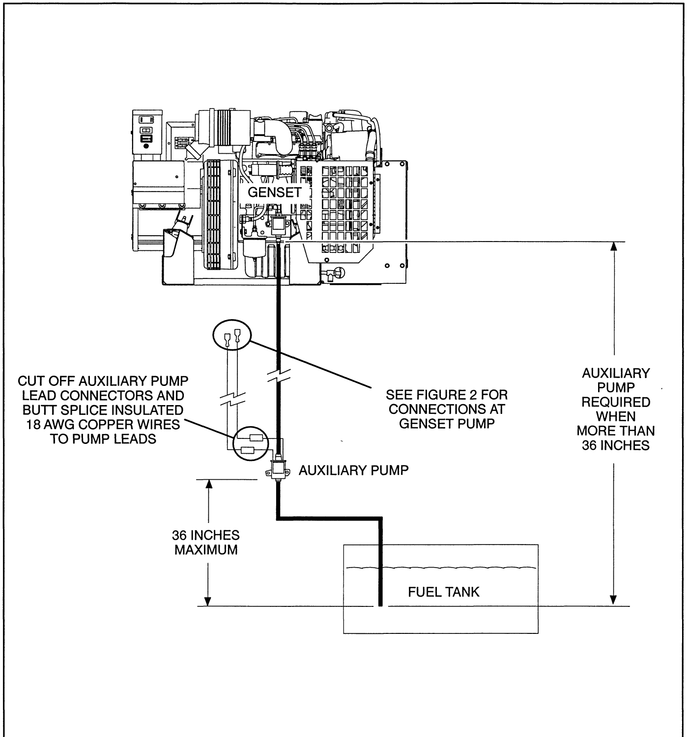
FIGURE 1. AUXILIARY PUMP INSTALLATION
