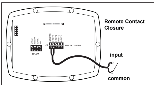
Figure 5. Connect to Remote Contacts
