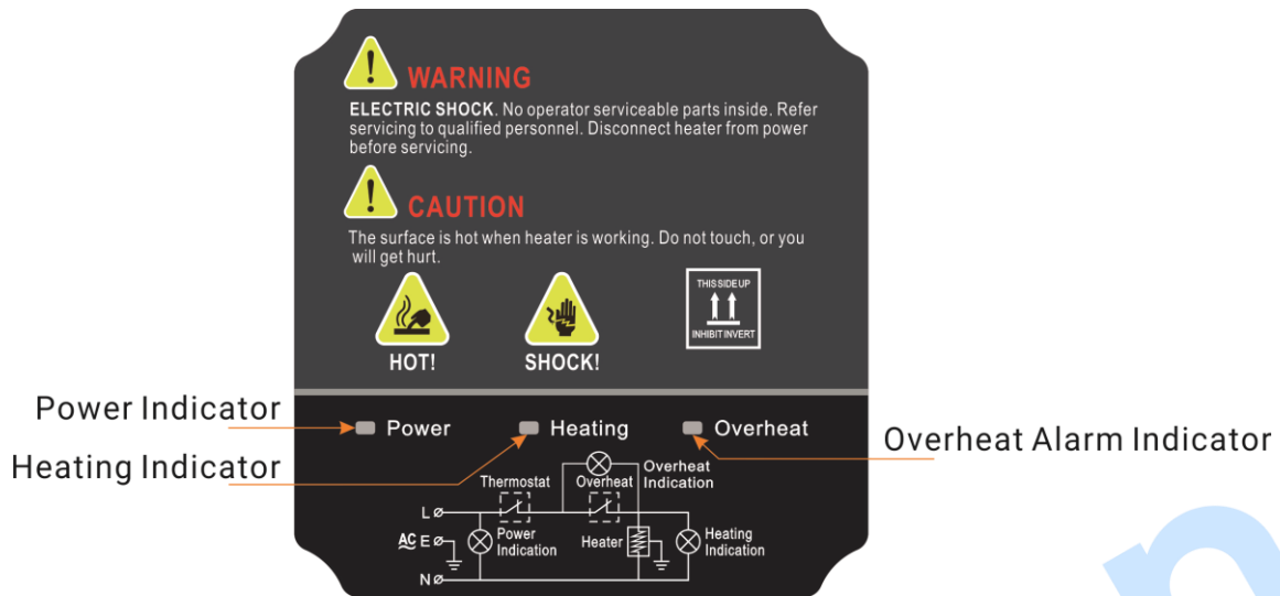
Fig.1 Panel Indication
