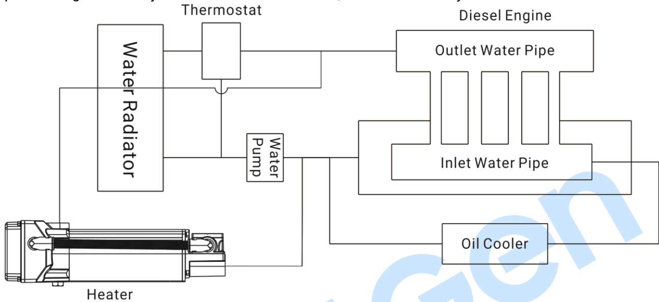
Fig.4 Working Diagram
