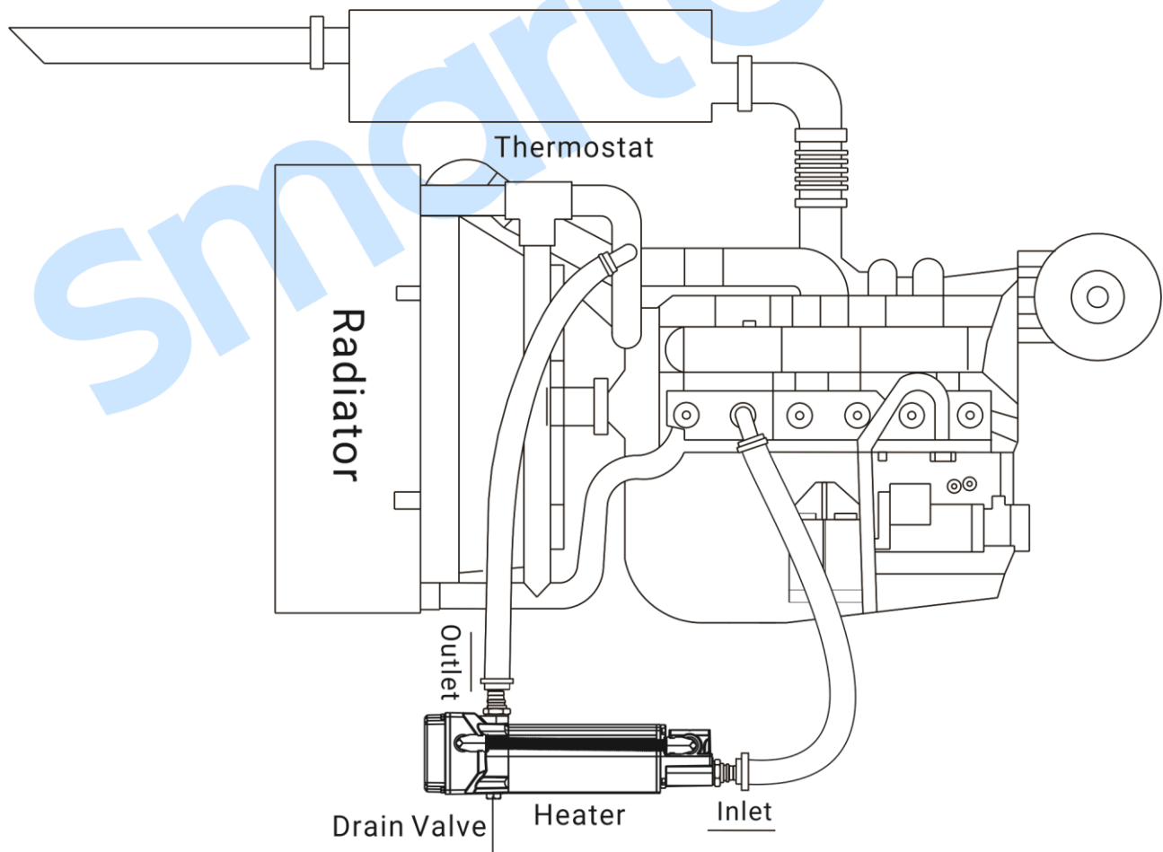
Fig.5 Installation Positions
