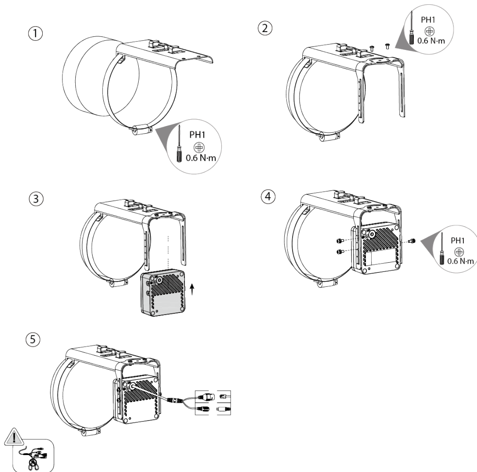
Figure 3-5 Attaching the Camera
