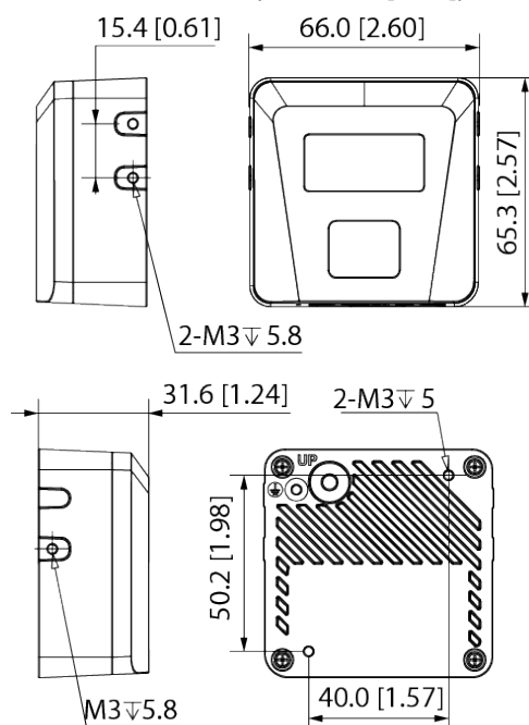
Figure 3-2 Dimensions (Unit: mm [inch])
