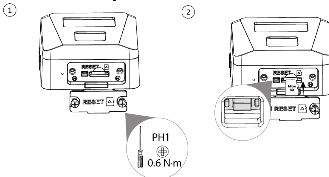
Figure 3-4 Install SD card
