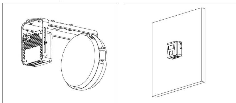
Figure 3-3 Installation methods
