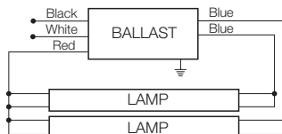
QUICKTRONIC 2x32
