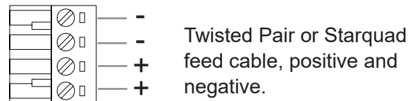
Figure 2: Output connections
