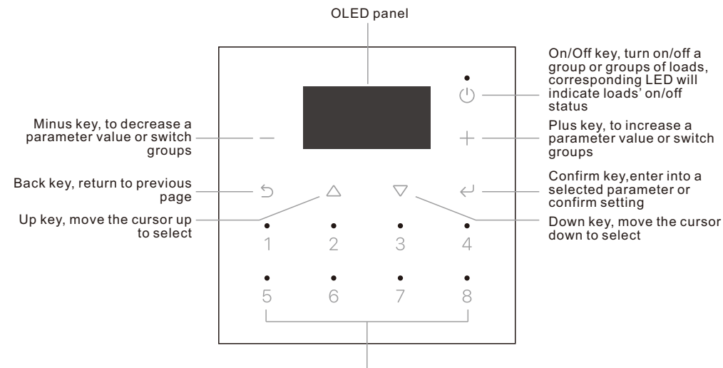
Front side
