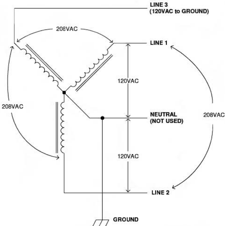
Figure 5. Wye Service Connections (Motiv drivetrain vehicles must use a Wye Service Connection)
