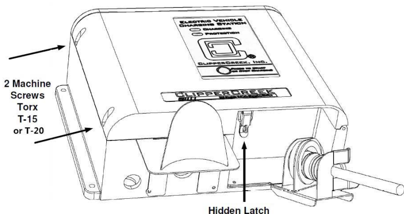
Figure 6. Front Door Hidden Latch
