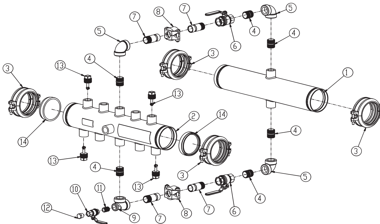
FIG. 1 PCMS ASSEMBLY
