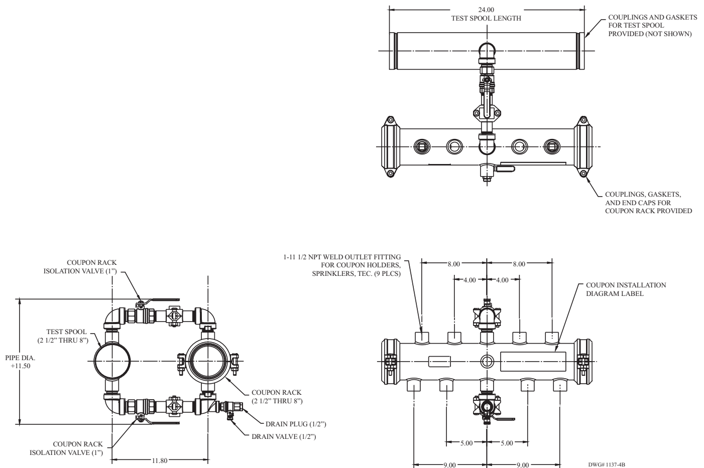
FIG. 4 PCMS OUTLINE DRAWING
