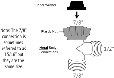
Hybrid Cold Water T-adapter (7/8" x 7/8" x 1/2")
