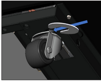
Fig. 7. Install shim(s).
