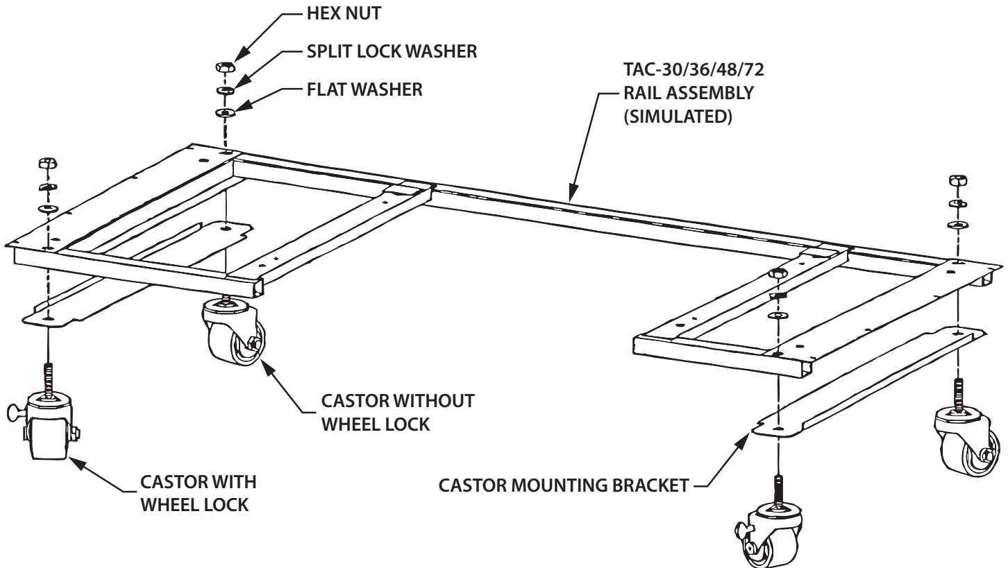
TAC-30/36/48/72 CASTOR KIT MOUNTING DIAGRAM
