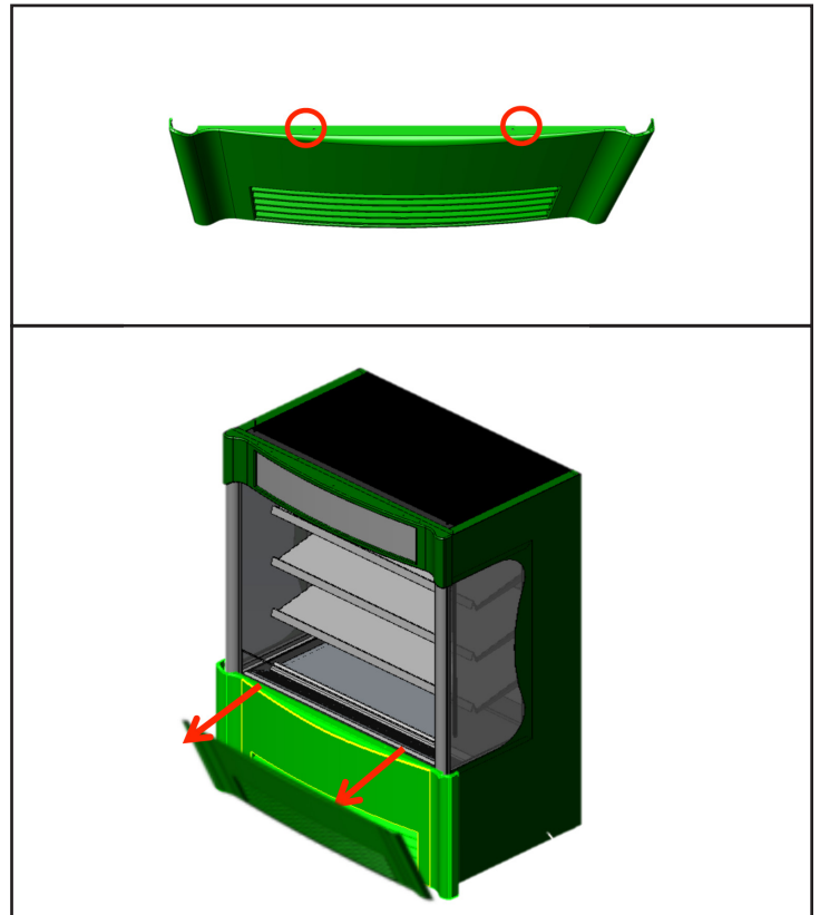
Fig. 3. TAC-48SM: Remove the screws and tilt the top of the grill forward.
