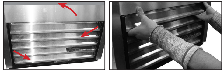
Fig. 1. Lower grill screw locations (A). Pull the grill from the cabinet front (B).
