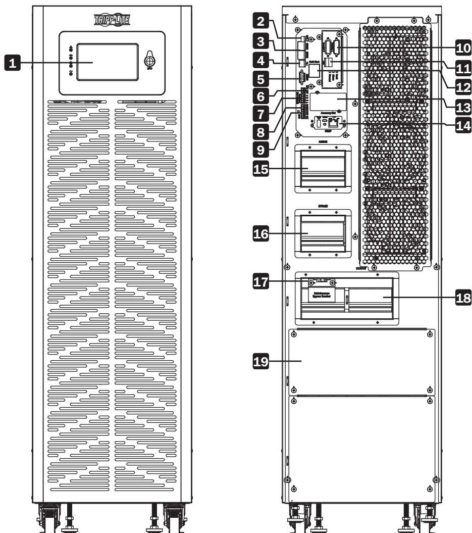
Figure 3-1: Front and Rear, Models S3M25K and S3M30K (see page 15 for callout explanation)
