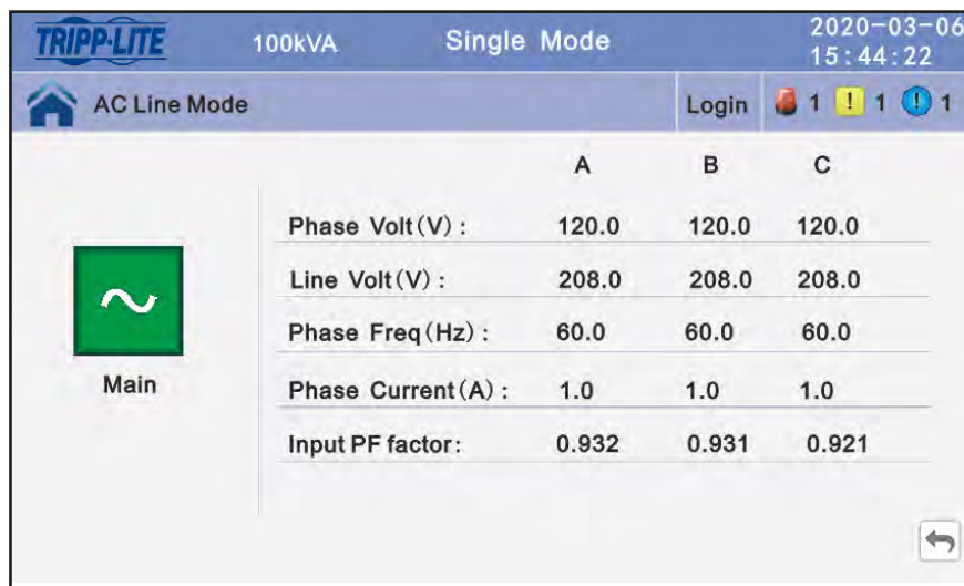
Figure 4-9: Main Data Display Window
