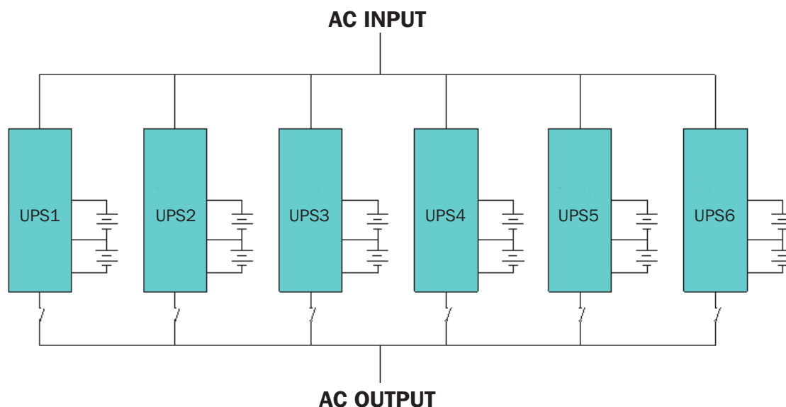
Figure 3-17: Connections for Parallel Installation
