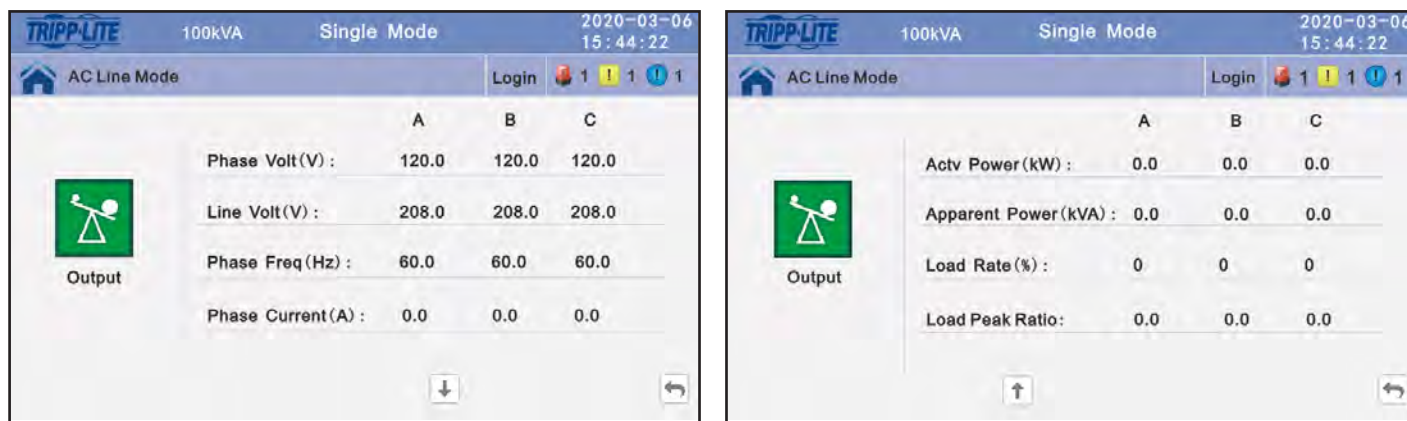
Figure 4-11: Output Data Display Window
