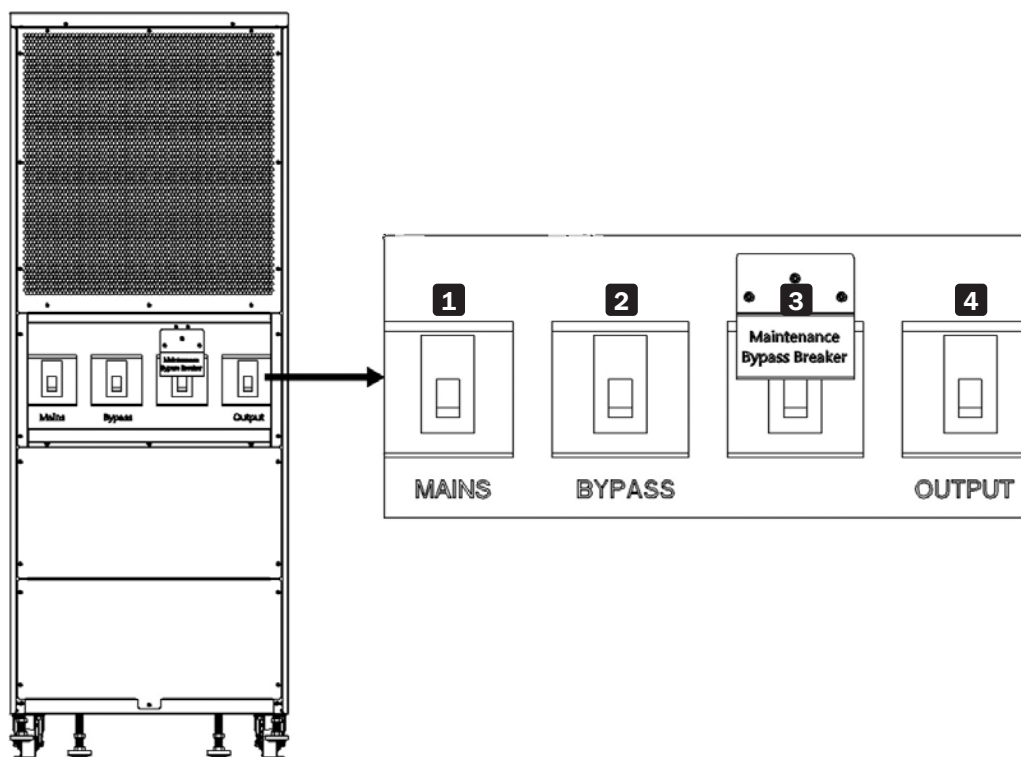
Figure 3-9: Rear View Detail, Models S3M80K and S3M100K
