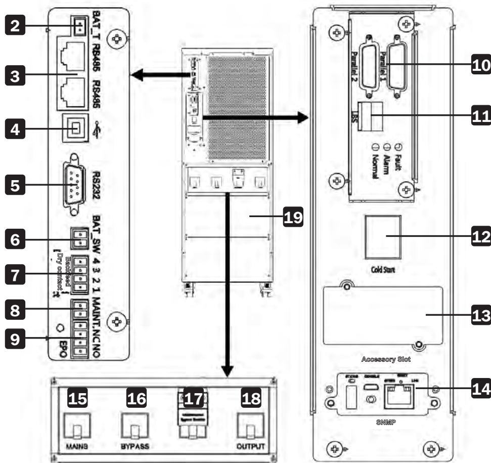
Figure 3-4: Rear View Detail, Models S3M50K and S3M60K
