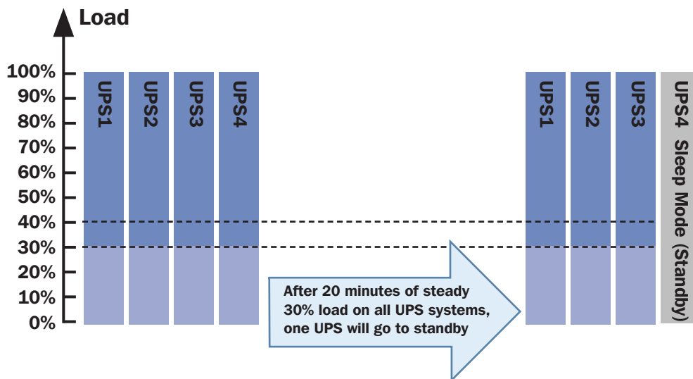
Figure 4-28D: Example, Inter Sleep Mode with Four UPS Systems
