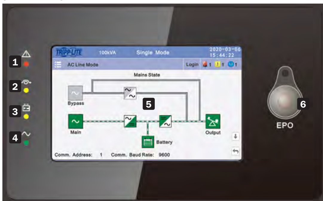
Figure 4-6: Overview of the operating panel of the UPS
