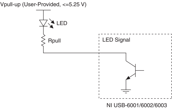
Figure 6. To Drive a Status LED
