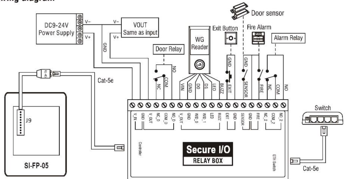
Wiring diagram
