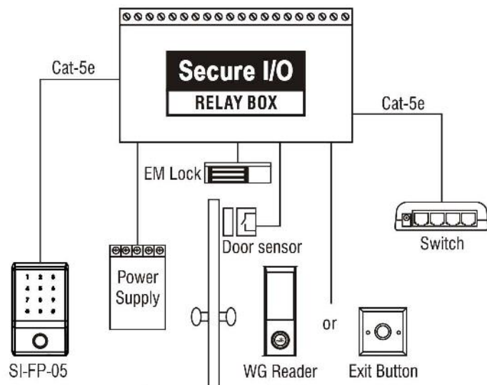
Structure (Standalone + Non POE version RELAY BOX)
