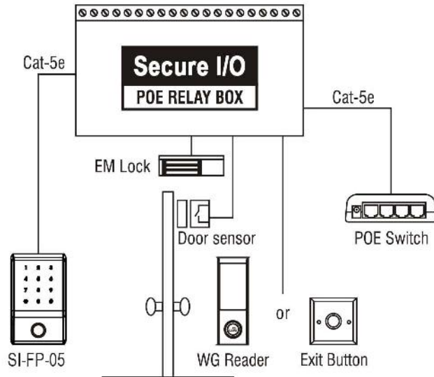
E. Structure (Standalone + POE version RELAY BOX)
