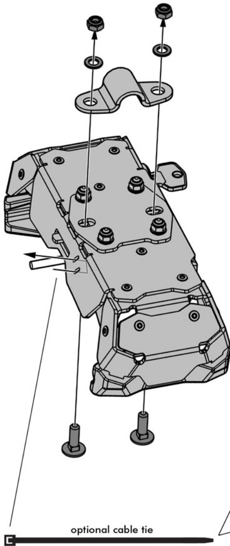
bracket 1
