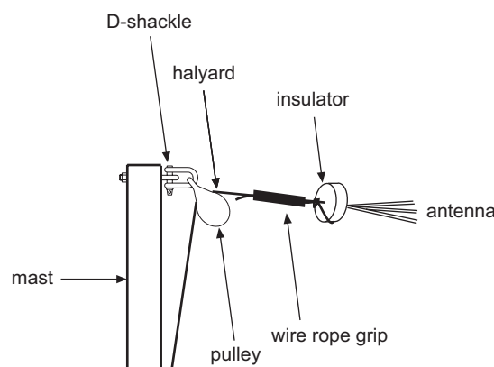
Figure 7: Masts and antenna
