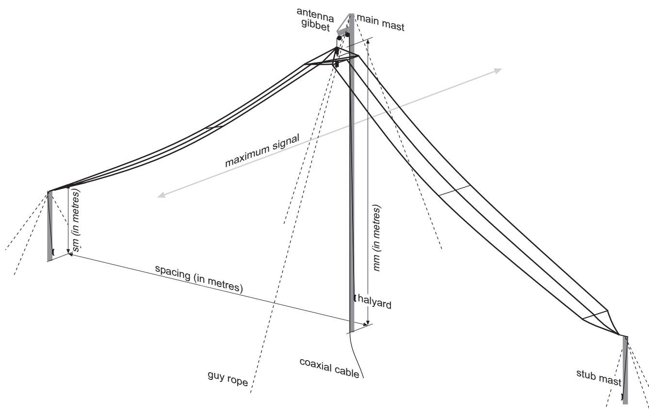
Figure 2: Inverted V configuration using the antenna gibbet
