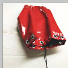
OUTLET For an air hose to supply fresh air or to extract dust from inside the tent. Item no. 6.400.000.027
