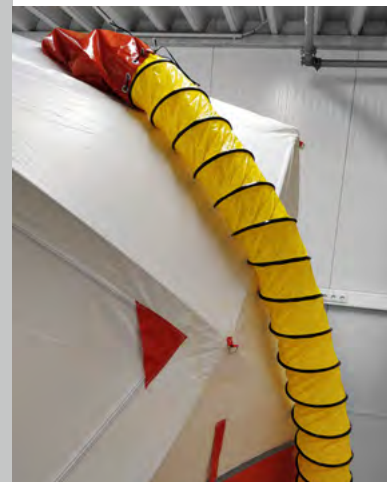
OUTLET For an air hose to supply fresh air or to extract dust from inside the tent. Item no. 6.400.000.027
