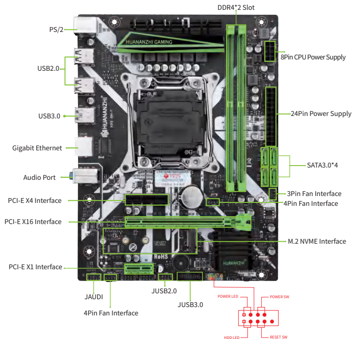
1-1 X99-8M F Motherboard Illustration
