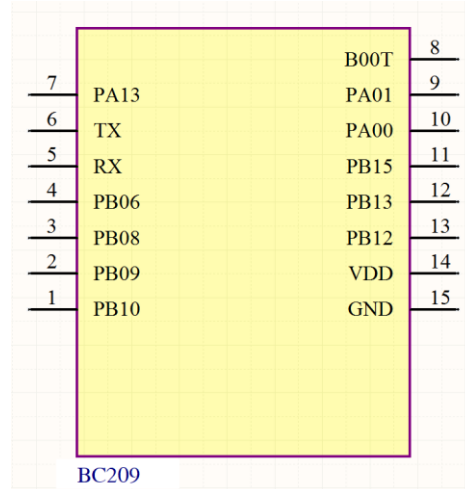
Fig 4.1 Pin Diagram
