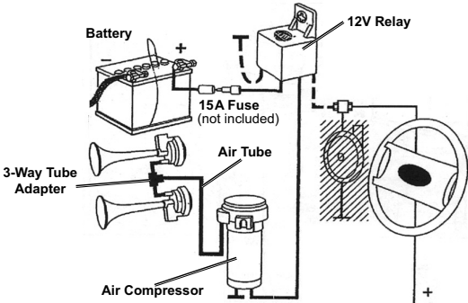
Negative Ground Wiring Diagram
