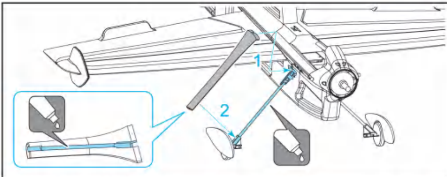
(22). 如图所示，装饰件蓝色部分需涂满泡沫胶才能牢固粘在碳杆上，先将右装饰件大头先装上，再装小头。 (装饰件有分左右方向，注意看装饰件卡口) Put on a foam coat on the right landing skid: seal the landing skid with glue as shown in figure, stick foam decorating parts with landing skid. (Stick the thick end of foam decorating parts firstly. Please well note the open end direction of foam decorating parts.)
