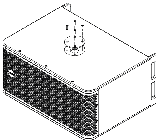
Figure 6.2: Cover plate removal
