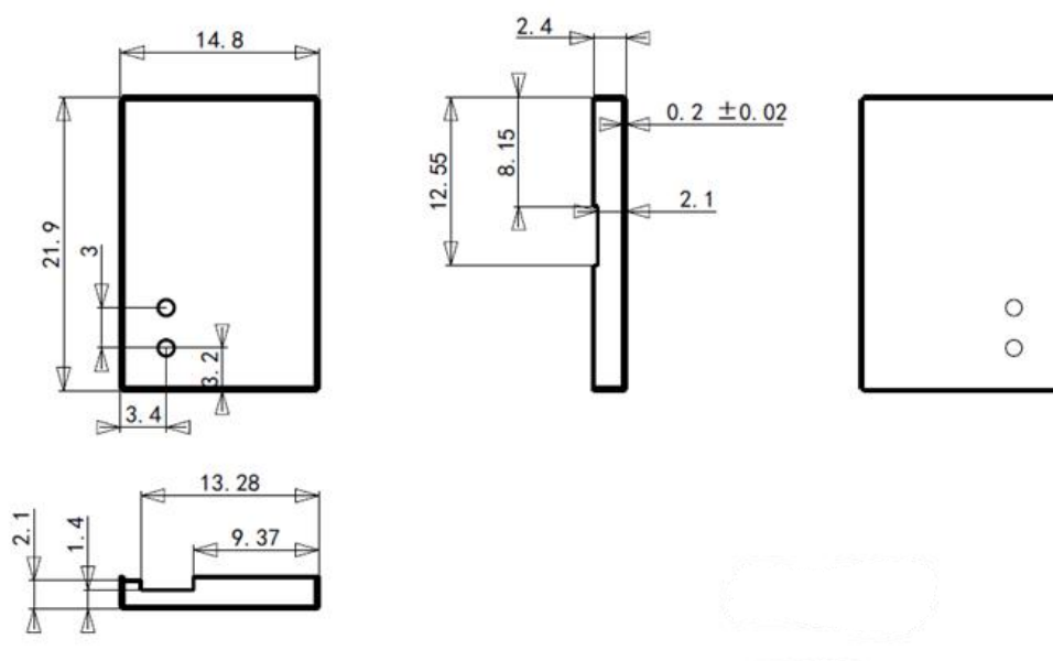
Fig 6 BL3372-P_1V1 Dimensions of shielding case
