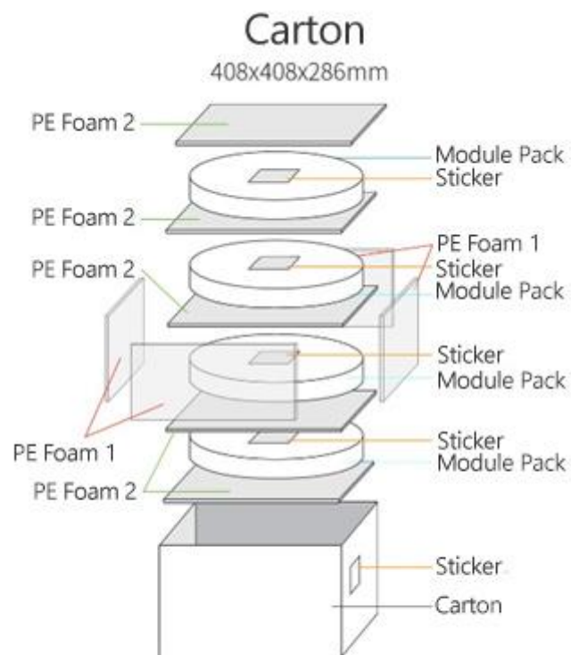
Fig 7 Packaging
