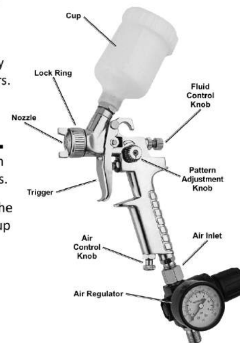
Figure C: Components & Controls
