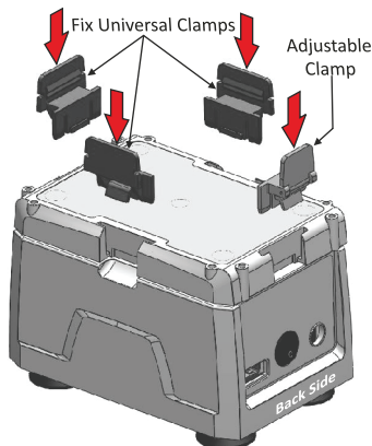
Installing Clamps
