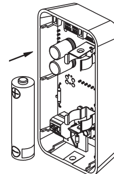
Fig. 6: Battery replacement
