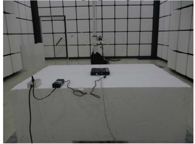
Part 15.247 2.4G Radiated Setup
