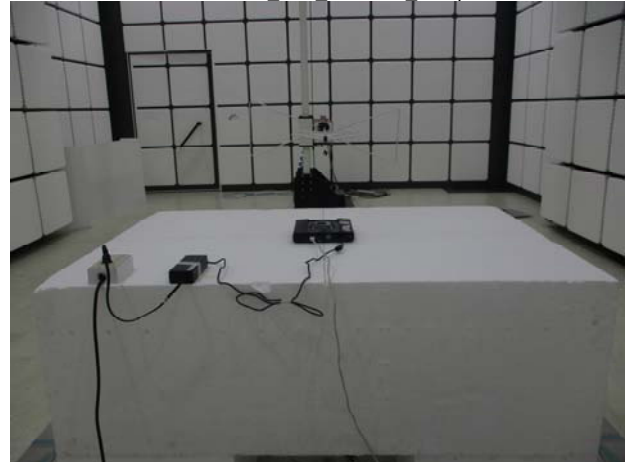
Part 15.247 BLE Radiated Setup
