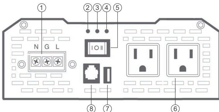
Figure 2: 1000W Inverter
