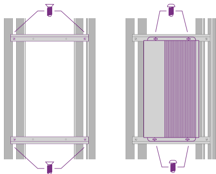
Round head screw - Driver to bracket
