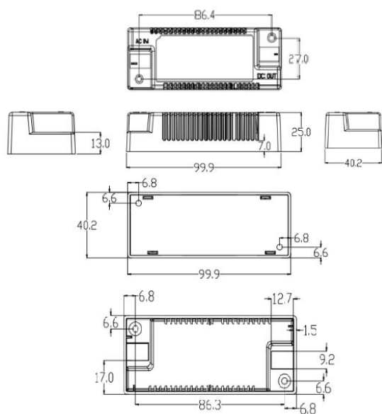
Full external casing version
