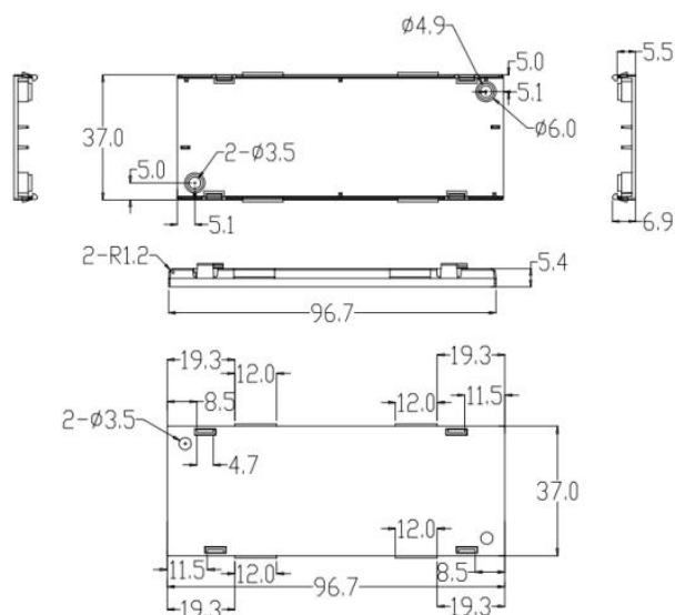
Bare board + fixed bottom casing version
