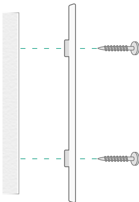
Wall Mounting Bracket
