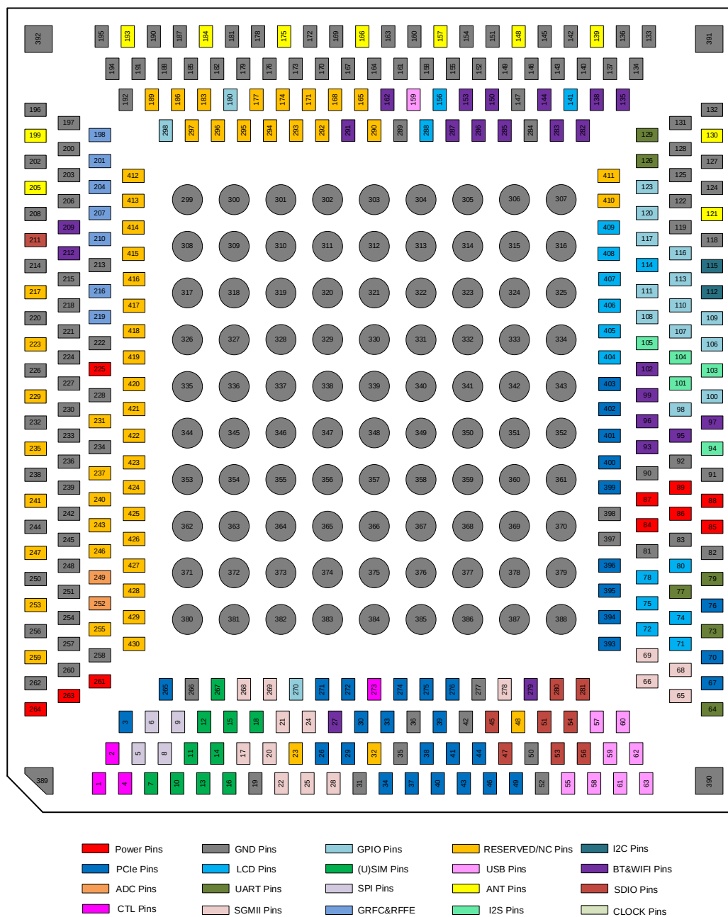
Figure 3-1 Pin map
