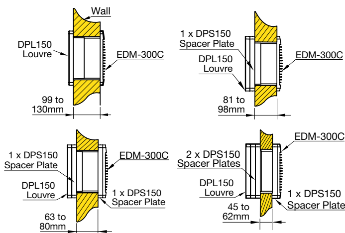
Spacer Plate (Model No: DPS150)
