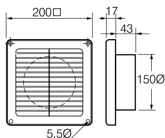
Slimfit Louvre Grille (Model No: DPL150)
