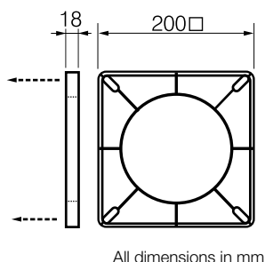
Spacer Plate (Model No: DPS150)
