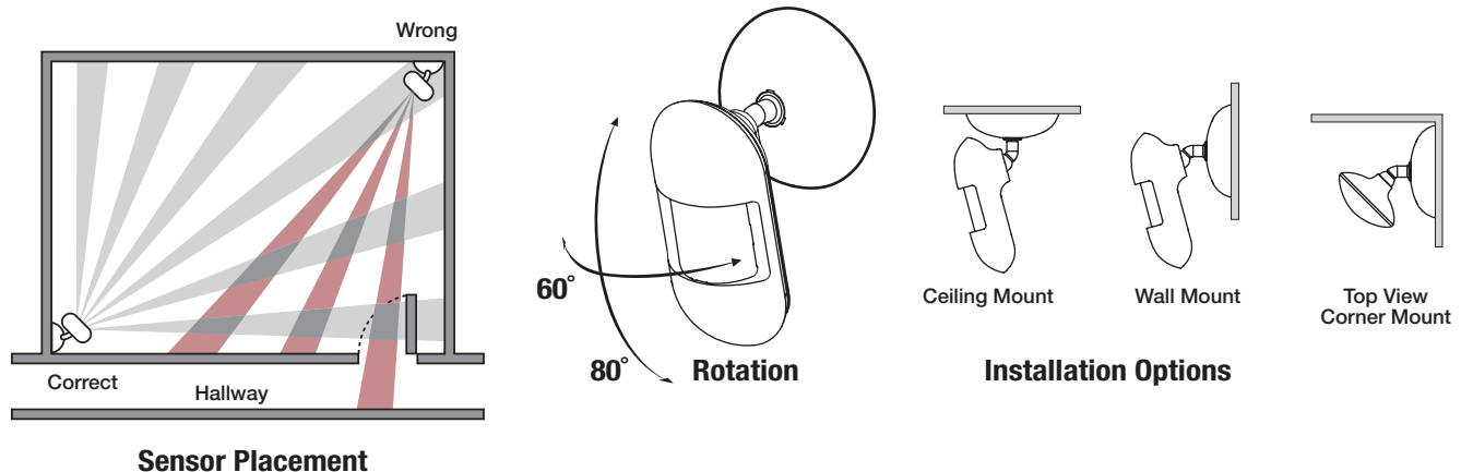
Figure 4. Sensor Placement and Installation Diagrams
