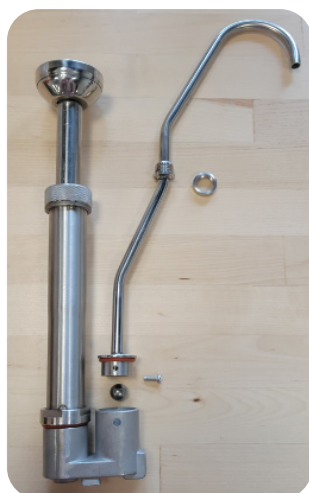
Pump Discharge Tube Unassembled
