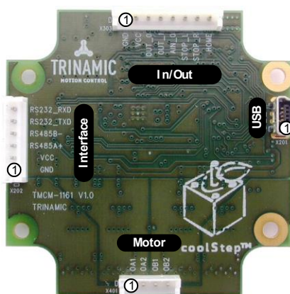
Figure 3.2 Overview connectors
