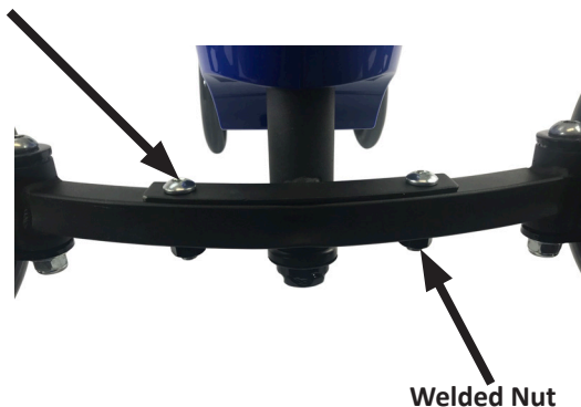
Front Axle Bolt
