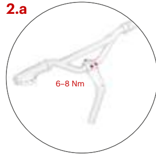
Handlebar installation
