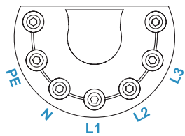
5 Wires: PE, Neutral, L1, L2, L3.
