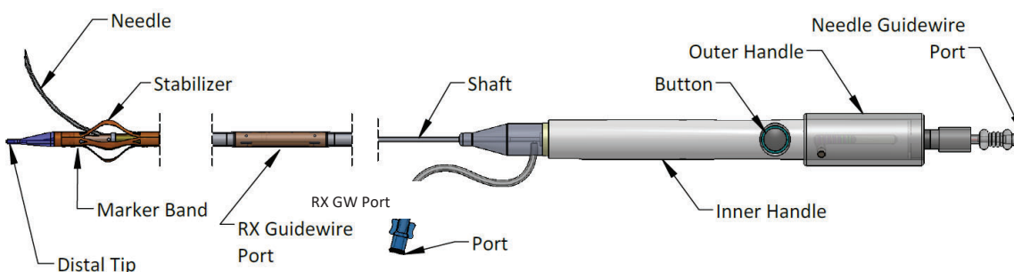
Figure 3: ENDOCROSS Device
