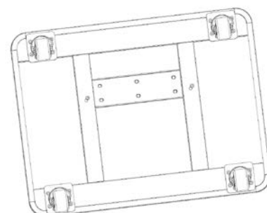
Figure 2-3 Secure coasters (3)
