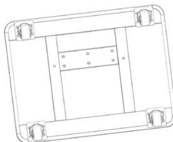
Figure 2-7 Secure bracket (4)
