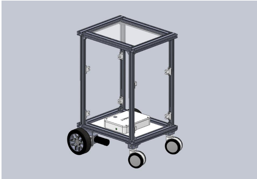
Fig. 18 Install the Controller box
