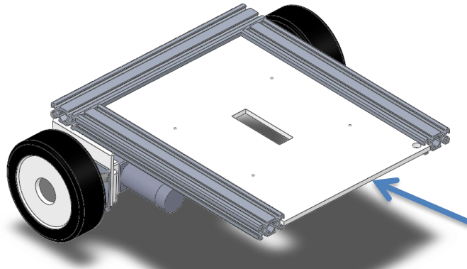
Fig. 10 Slide in the Bottom Plate
