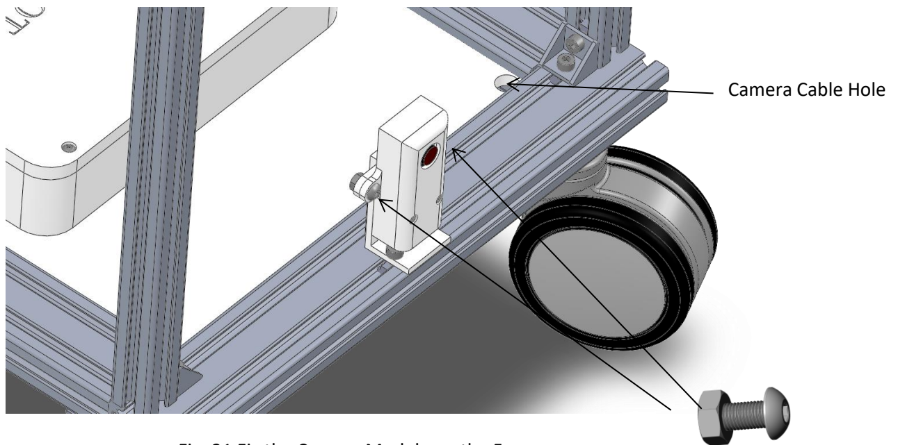
Fig. 21 Fix the Camera Module on the Frame
