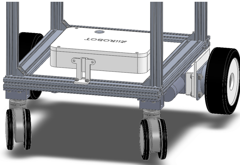
Fig. 20 Fix the Camera Frame on the Front Aluminum Extrusion
