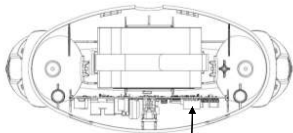
battery connector
