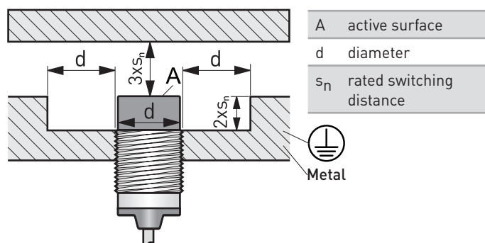
III. 1: Free space around a cylindric non-flush wireless inductive sensor and distance to an opposite conductive surface.
